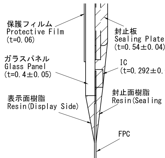
B部拡大図 (10 : 1) B-Portion Magnified Drawing (10:1)
