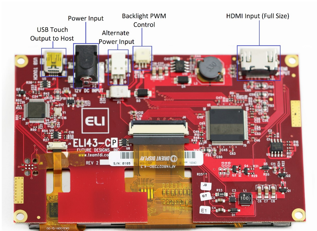
Figure 3. ELI43-CP Connectors
