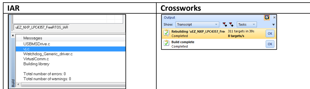
Figure 9: Build Finished
