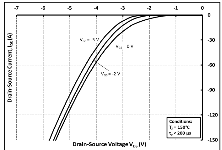
Figure 10. Body Diode Characteristic at 150\text{ °C}
