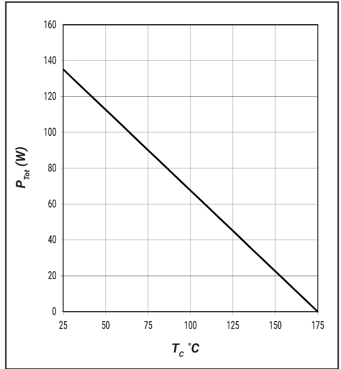
Figure 4. Power Derating
