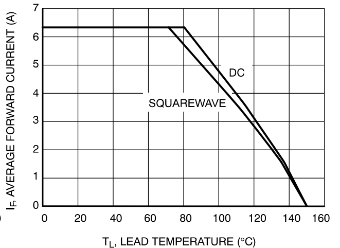
Figure 6. Derating Curve
