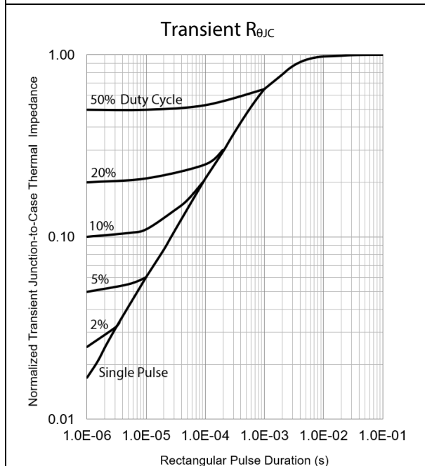
1.00 = Nominal DC thermal impedance
