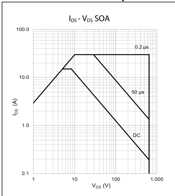
Figure 13: Safe Operating Area @ T_{case} = 25\text{ }^{\circ}C
