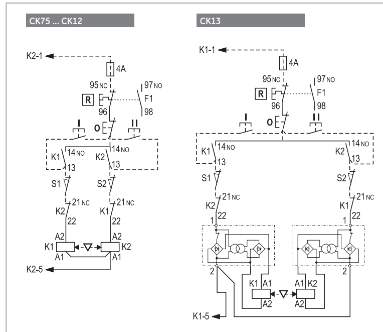
Control circuit
