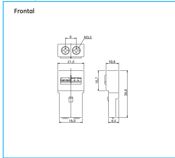
Alarm contact blocks
