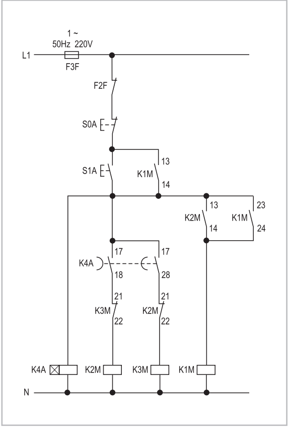
Control circuit
