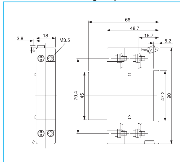
Shunt and undervoltage trip devices
