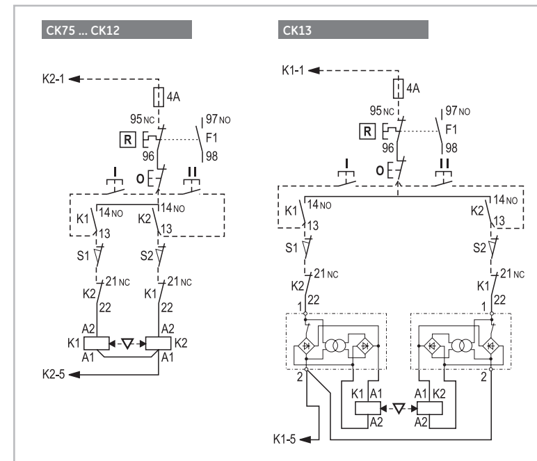
Control circuit
