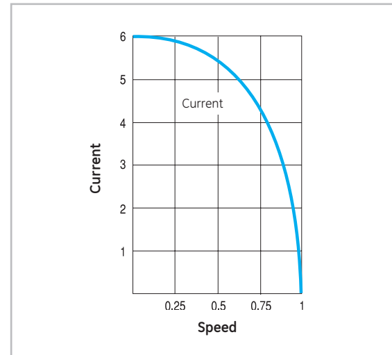
Current-speed curve
