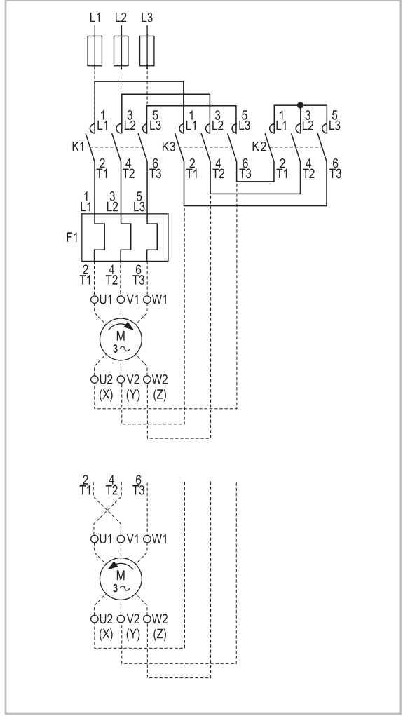
Power circuit
