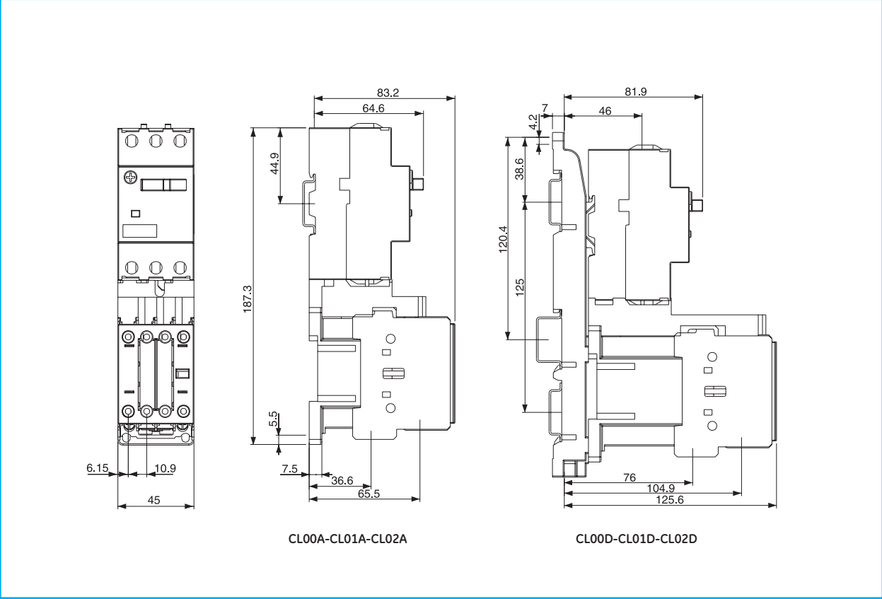
Fuseless starter - GPS1 rocker + Contactor CL00-CL01-CL02
