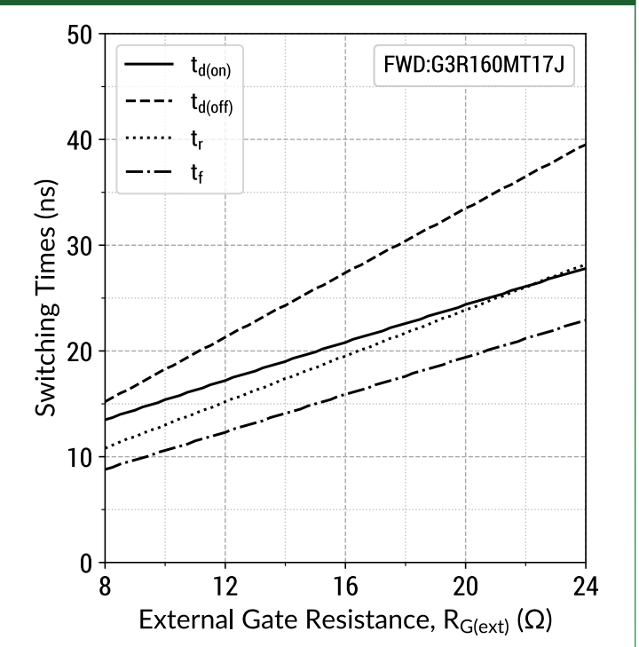
Figure 24: Switching Time v/s R_{G(ext)} ( V_{DD} = 1200V )
