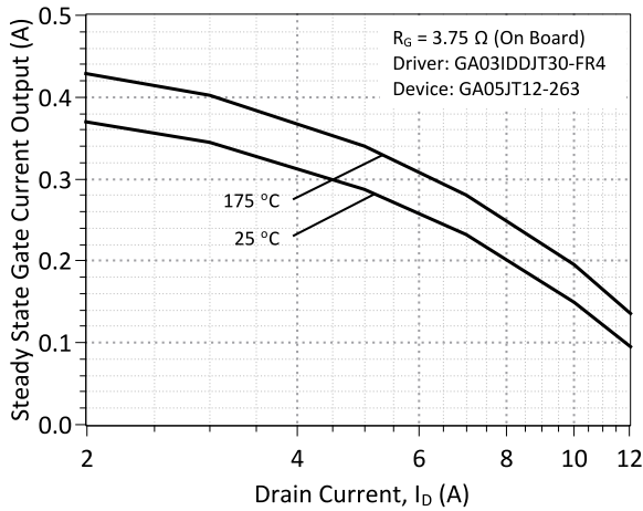
Figure 24: Typical steady state gate current supplied by the GA03IDDJT30-FR4 board for the GA05JT12-263 with the on board resistance of 3.75 Ω
