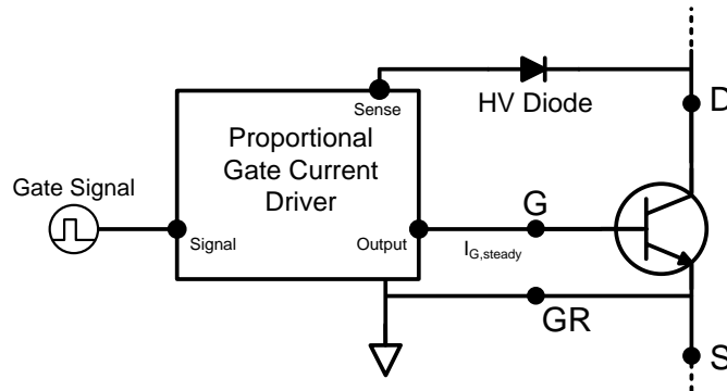
Figure 27: Simplified Voltage Controlled Proportional Driver
