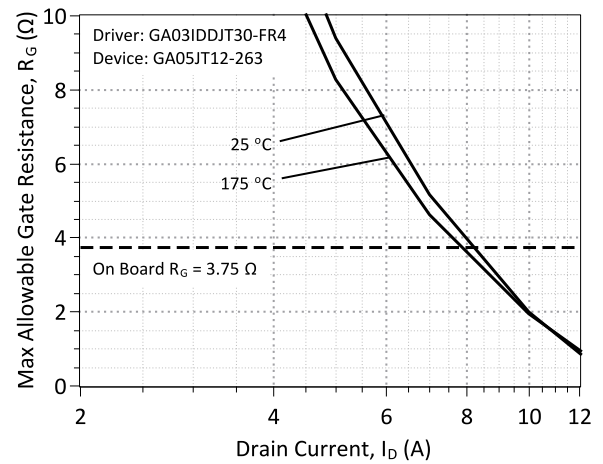
Figure 25: Maximum gate resistance for safe operation of the GA05JT12-263 at different drain currents using the GA03IDDJT30-FR4 board.
