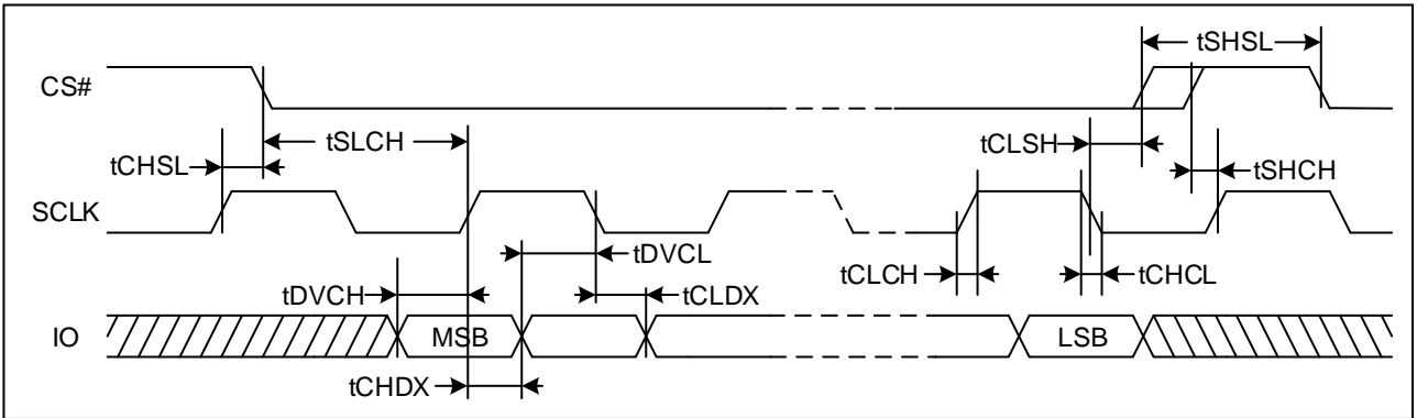
Figure 95. Serial Input Timing (DTR)
