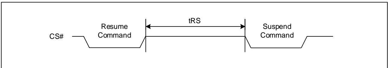
Figure 97. Resume to Suspend Timing Diagram
