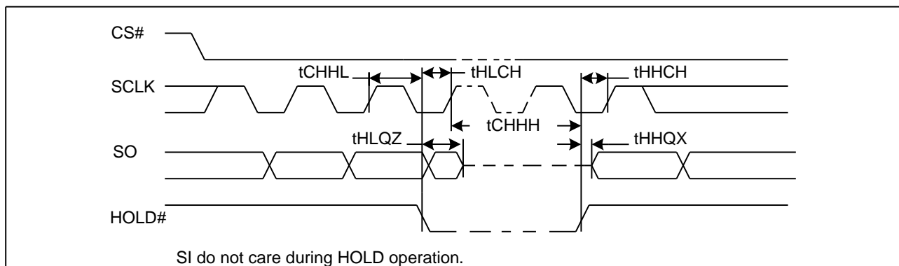
Figure 81 Hold Timing
