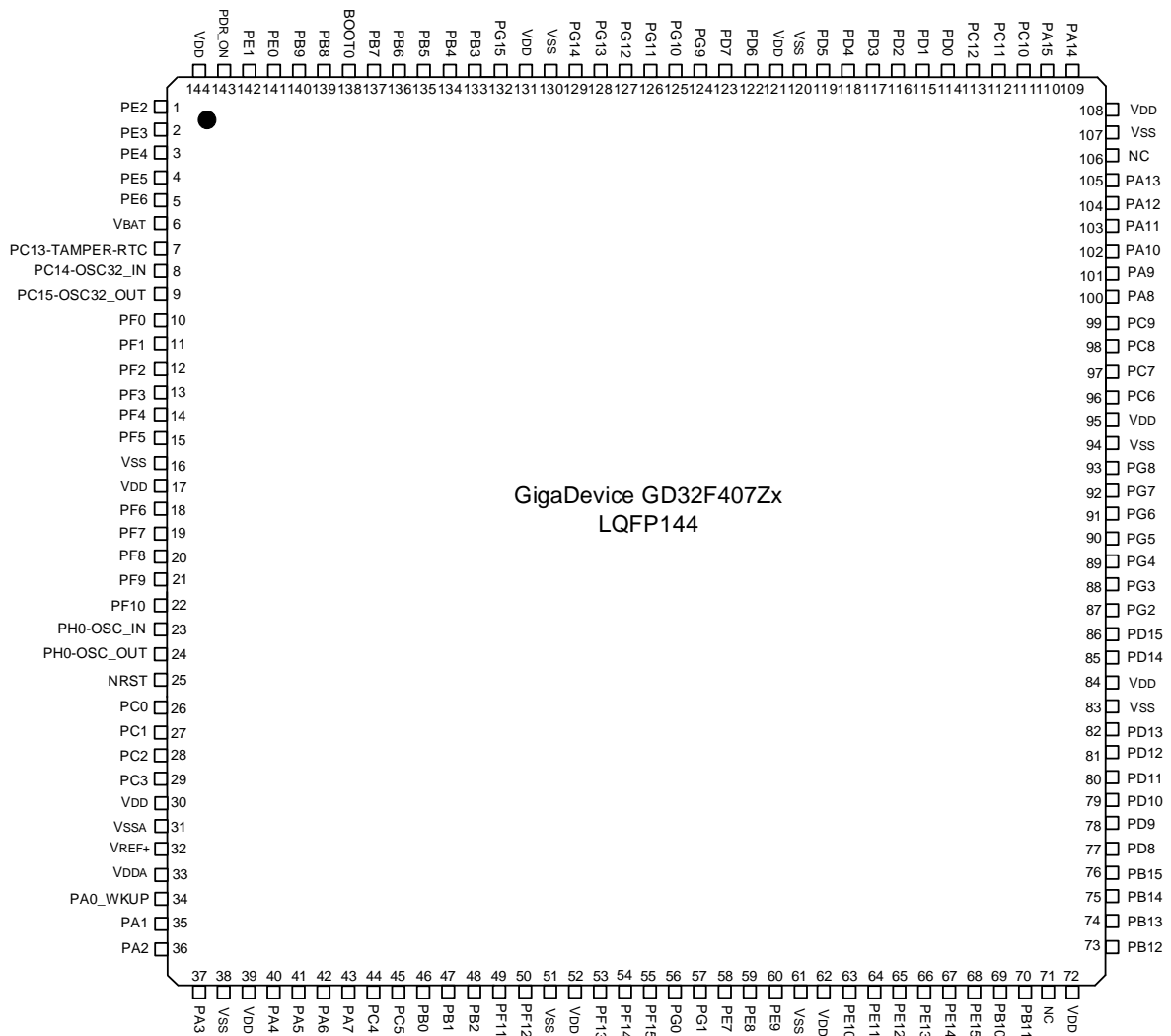
Figure 4. GD32F407Zx LQFP144 pinouts
