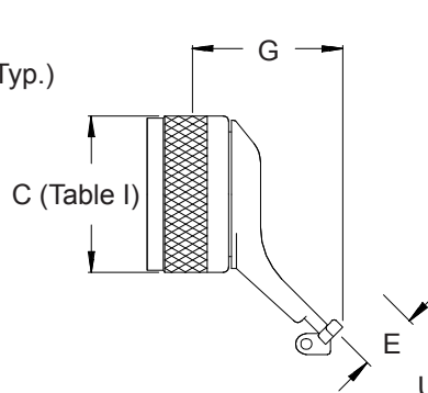
45° ROTATABLE COUPLING
