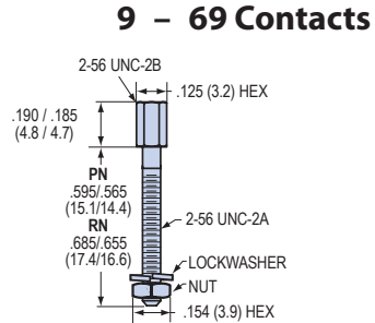
PN Kit Part Number 500-069-2-6 RN Kit Part Number 500-069-2-7 Kit Consists of 2 Jackposts, 2 Nuts, 2 Washers
