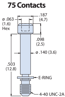
Kit Part Number 500-080-3 Kit Consists of 2 Jackscrews and 2 E-Rings
