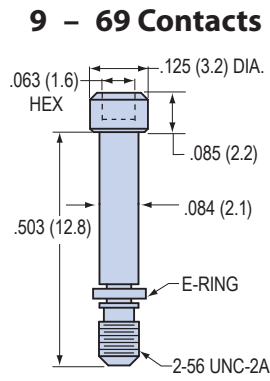
Kit Part Number 500-080-2 Kit Consists of 2 Jackscrews and 2 E-Rings
