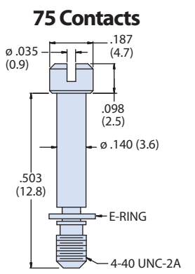
Kit Part Number 500-081-3 Kit Consists of 2 Jackscrews and 2 E-Rings
