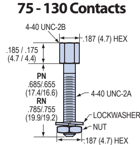
PN Kit Part Number 500-069-4-7 RN Kit Part Number 500-069-4-8 Kit Consists of 2 Jackposts, 2 Nuts, 2 Washers
