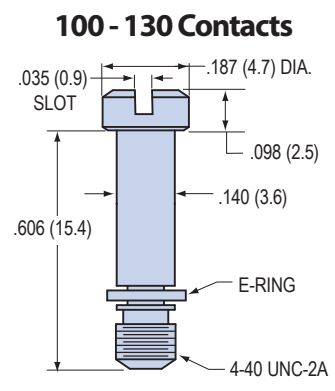
Kit Part Number 500-081-4 Kit Consists of 2 Jackscrews and 2 E-Rings
