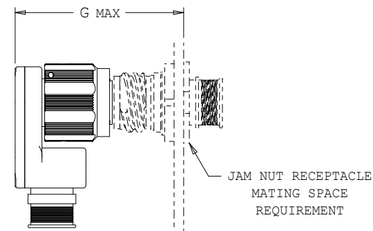
SQUARE FLANGE RECEPTACLE MATING SPACE REQUIREMENT
