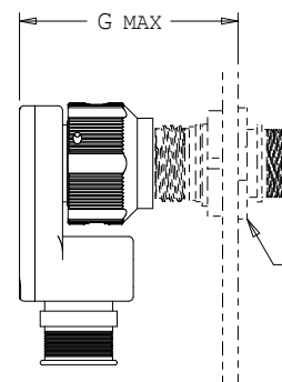
SQUARE FLANGE RECEPTACLE MATING SPACE REQUIREMENT
