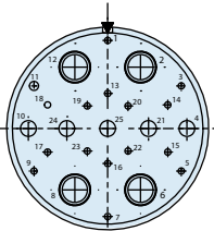
Arrangement 25L-26 (IAW PREN 3645-001) 16x Size 20 5x Size 12 4x Size 8
