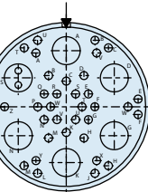
Arrangement 25Q-17 36x Size 22 6x Size 8
