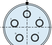
Arrangement 23L-05 (IAW PREN 3645-001) 5x Size 8
