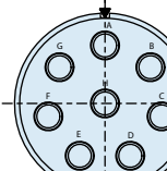
Arrangement 25L-08 8x Size 8
