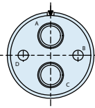
Arrangement 17I-22 (IAW PREN 3645-001) 2x Size 8 2x Size 12
