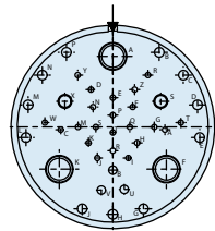
Arrangement 25L-41 22x Size 22d 3x Size 20 11x Size 16 2x Size 12 3x Size 8
