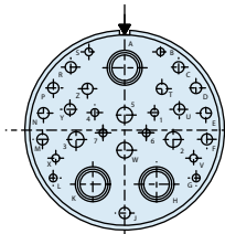
Arrangement 25I-20 (IAW PREN 3645-001) 10x Size 20 13x Size 16 4x Size 12 3x Size 8
