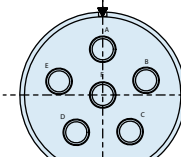
Arrangement 23L-06 (IAW PREN 3645-001) 6x Size 8
