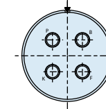
Arrangement 19L-04 4x Size 8
