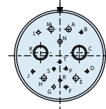
Arrangement 19L-17 10x Size 22d 1x Size 20 4x Size 16 2x Size 8
