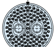
Arrangement 25L-07 97x Size 22 2x Size 8
