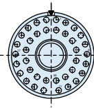
Arrangement 17I-02 1x Size 8 38x Size 22
