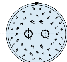
Arrangement 25L-46 40x Size 20 4x Size 16 2x Size 8
