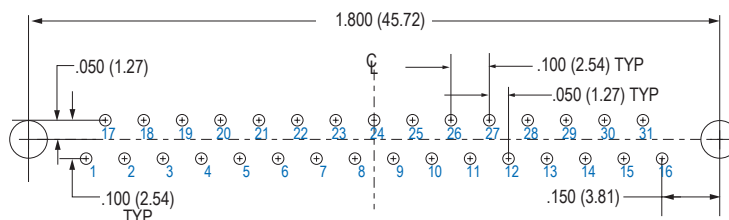
31 SOCKET M83513/25-E
