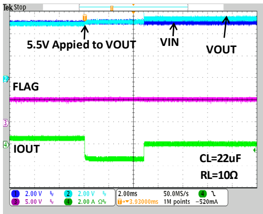
Reverse-Voltage Protection Response
