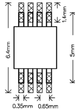
MSOP-8
