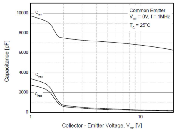
Fig. 6 Capacitance characteristics
