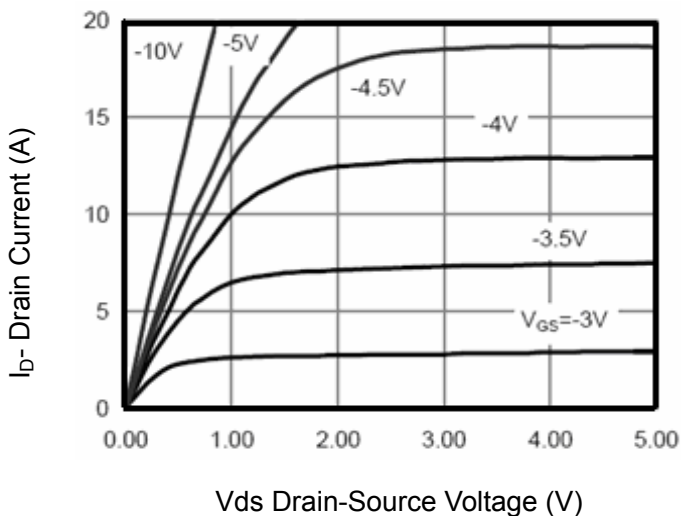
Figure 5 Output CHARACTERISTICS
