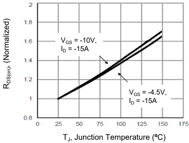
Figure 7. Drain-Source On-Resistance
