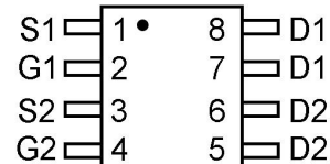
pin assignment
