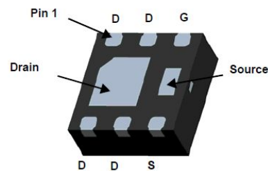
DFN2*2-6L
