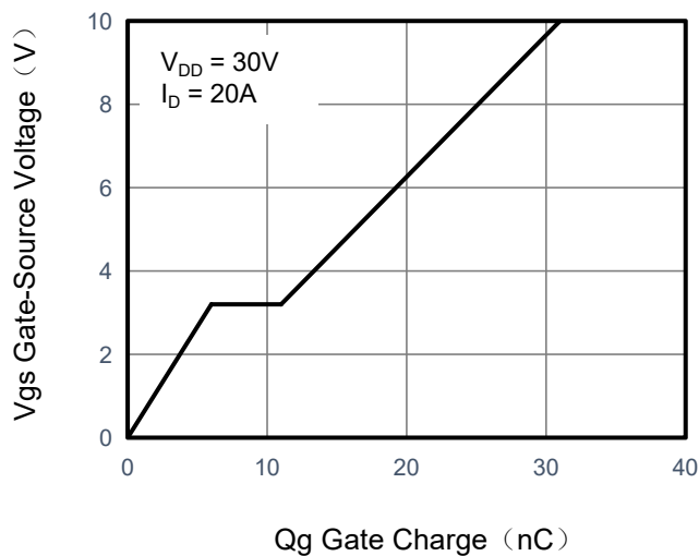
Figure 4. Gate Charge
