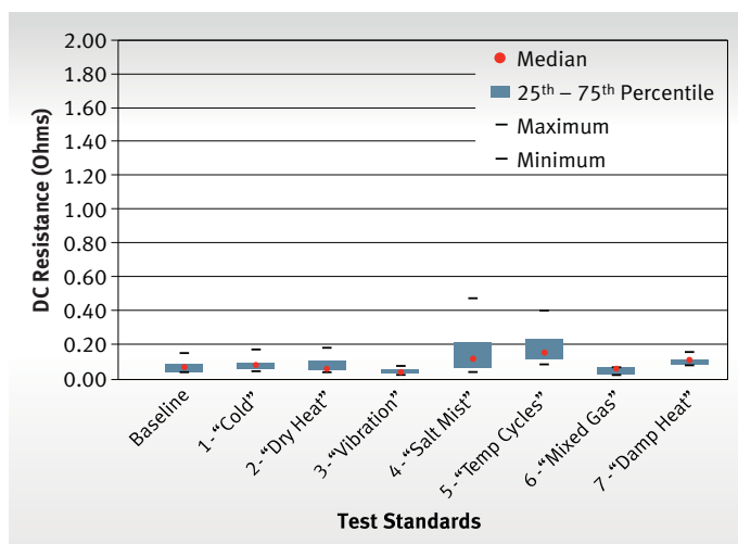
FIGURE 9: DC RESISTANCE THROUGH ALT FOR 1.30 MM SMT GS5200 SERIES PARTS
