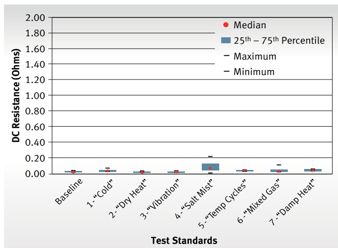
FIGURE 7: DC RESISTANCE THROUGH ALT FOR 0.72 MM SMT GS5200 SERIES PARTS
