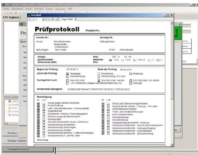
Report Generating
