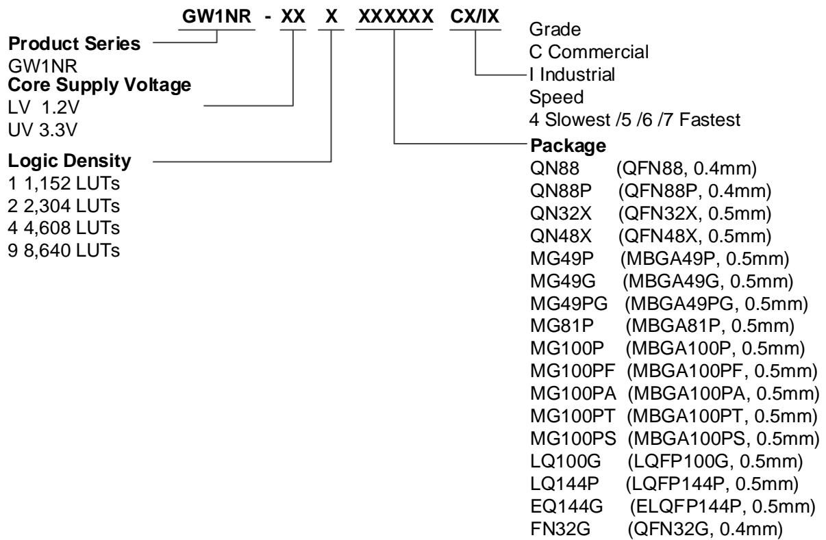
Figure 5-2 Part Naming-Production
