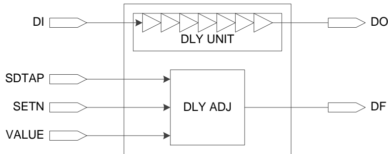
Figure 3-11 IODELAY
