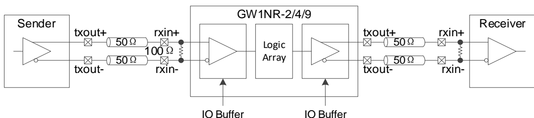
Figure 3-8 True LVDS Design
