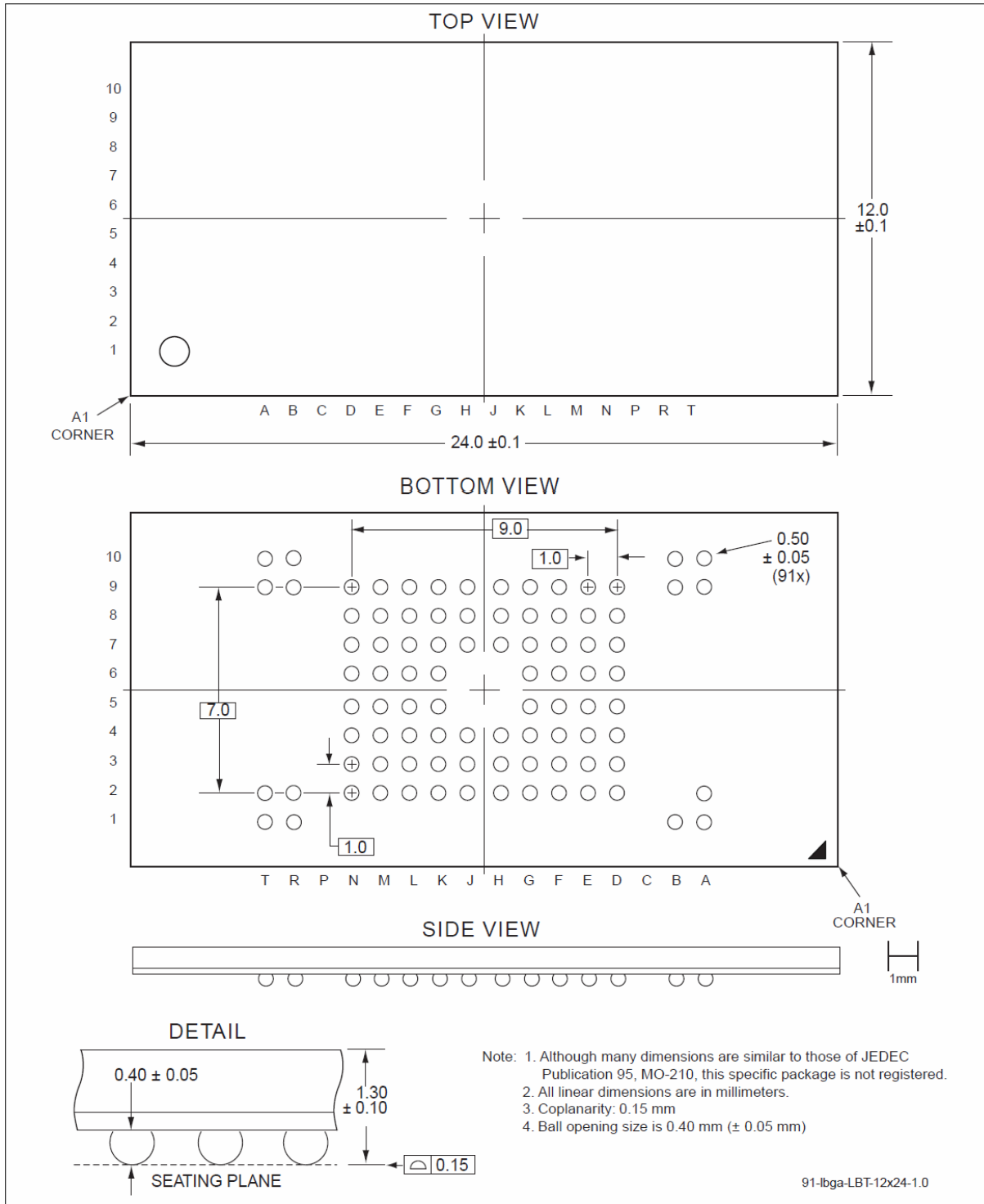
Figure 12-3: PATA NANDrive 91-Ball, Ball Grid Array (BGA) Greenliant Package Code: LBTE
