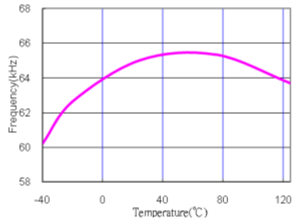
Fig. 4 CCM Frequency (kHz) vs. Temperature
