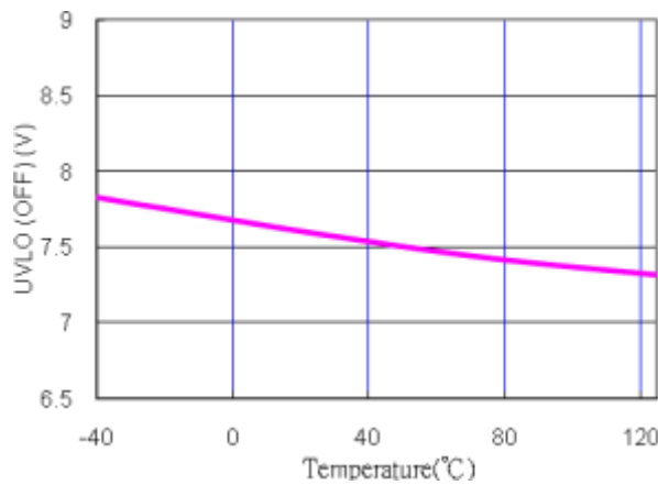
Fig. 3 UVLO (OFF) (V) vs. Temperature
