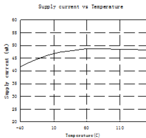
V_{OUT}=2.5V, I_{OUT}=1mA, V_{DD}=3.5V
