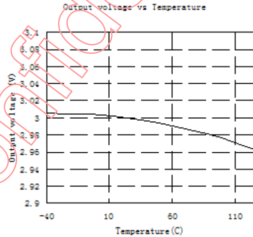
V_{OUT}=3.0V, I_{OUT}=1mA, V_{DD}=4.0V
