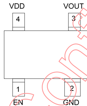
Figure 3c SC-82 Package
