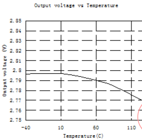
V_{OUT}=2.8V, I_{OUT}=1mA, V_{DD}=3.8V
