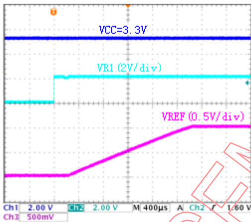
V_{CC}=3.3V , V_{REF}=1V , No Load Power On from EN
