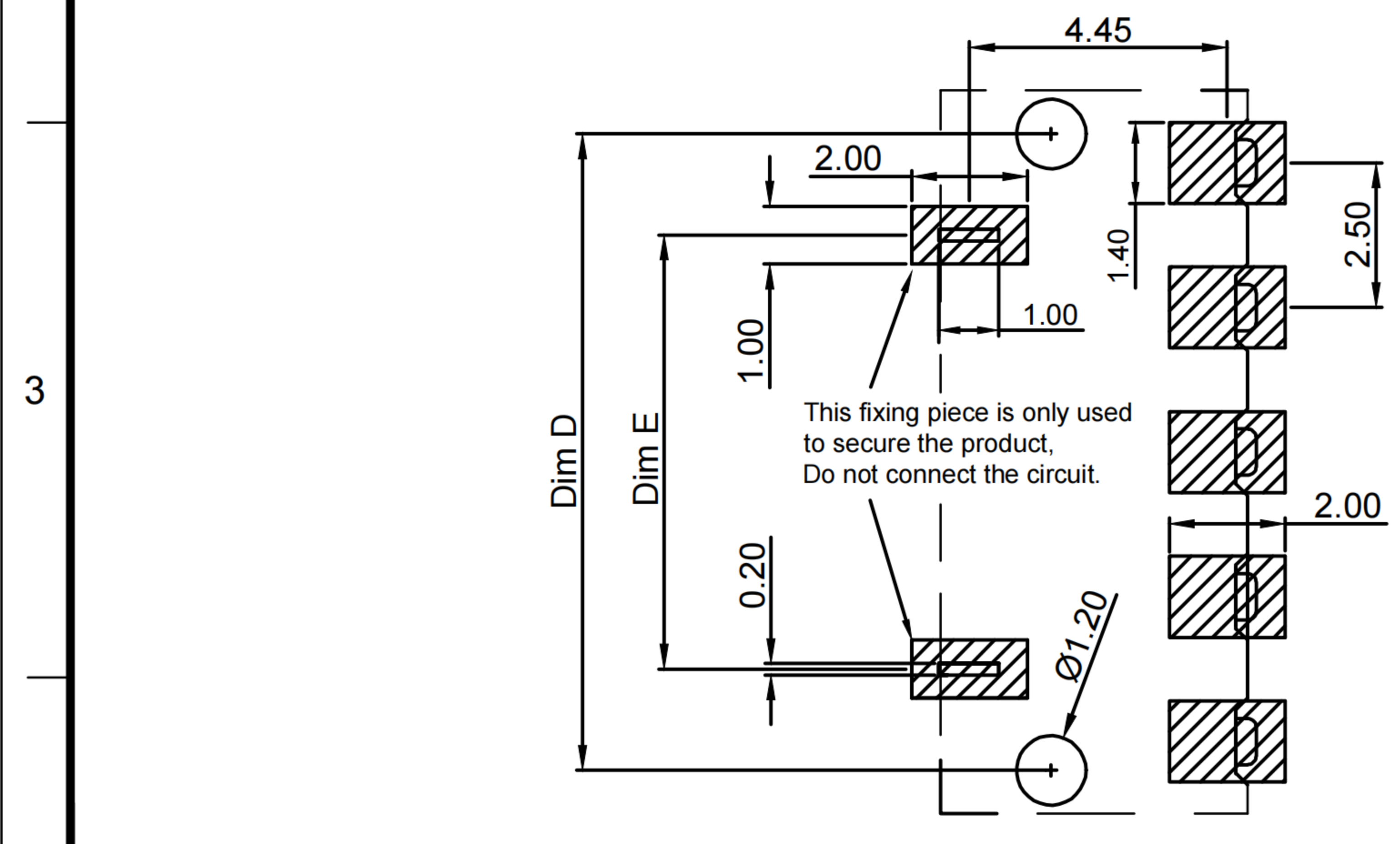
RECOMMENDED PCB LAYOUT TOLERANCE: ±0.05
