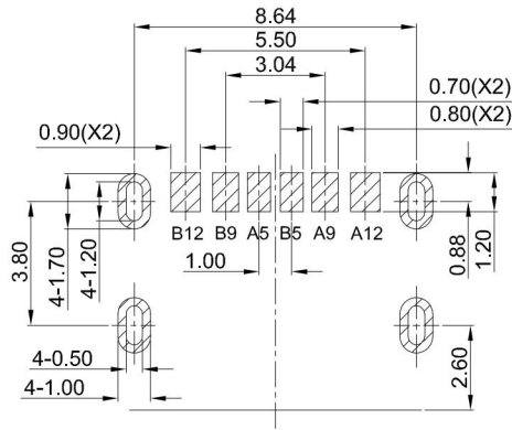
RECOMMENDED P.C.B. LAYOUT TOLERANCE ±0.05mm
