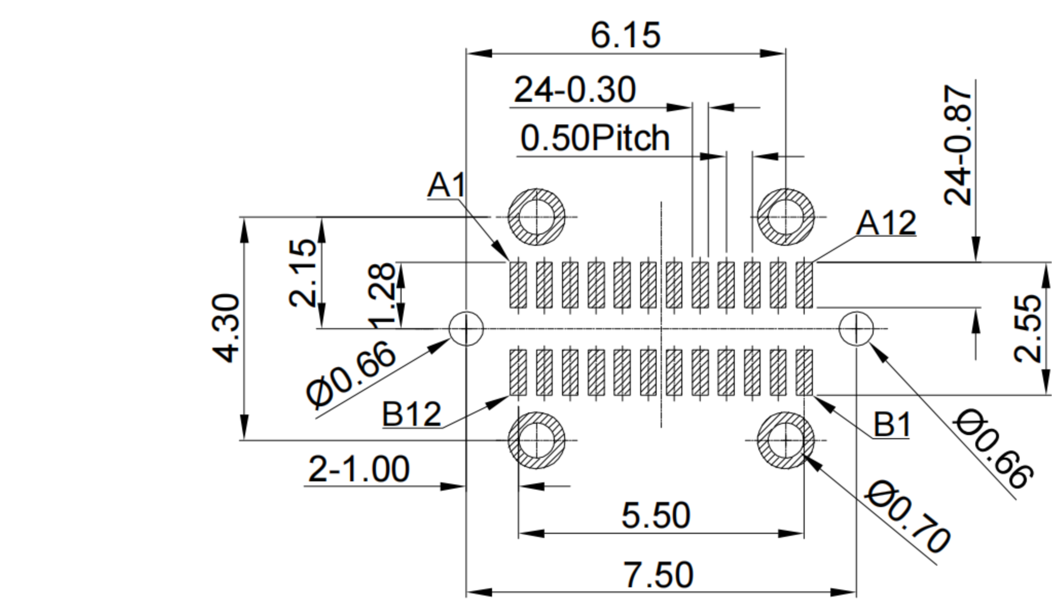
RECOMMENDED P.C.B. LAYOUT TOLERANCE UNSPECIFIED ±0.05mm
