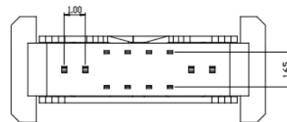
RECOMMENDED P.C.B. LAYOUT (T:1.00mm) TOLERANCE UNSPECIFIED ±0.05mm
