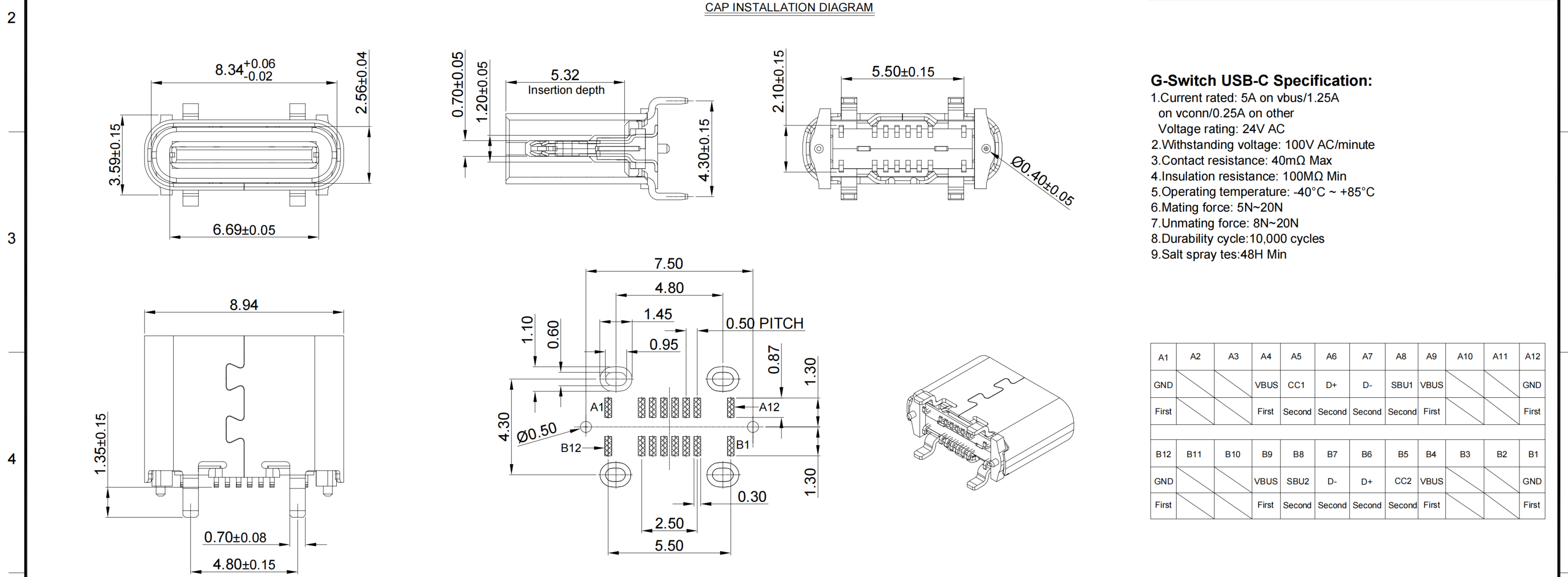
RECOMMENDED PCB LAYOUT TOLERANCE:±0.05
