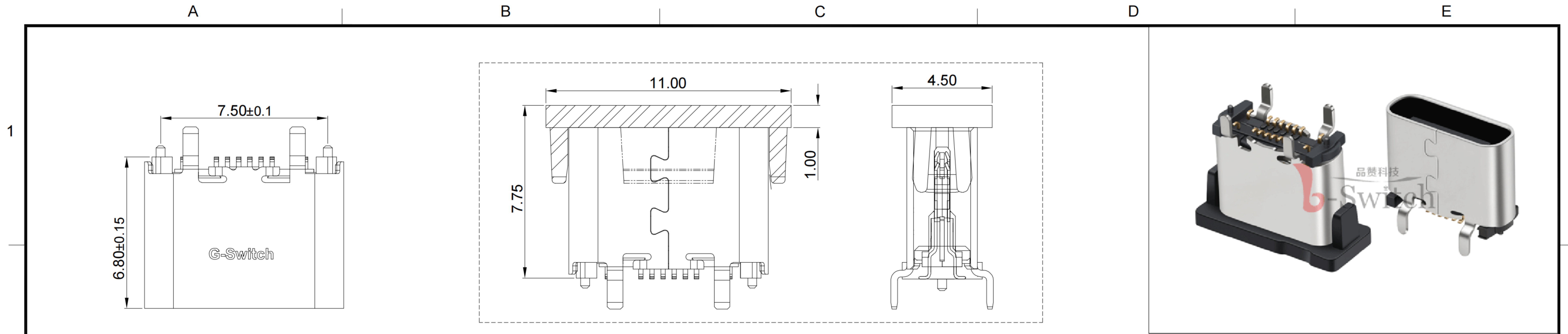
CAP INSTALLATION DIAGRAM
