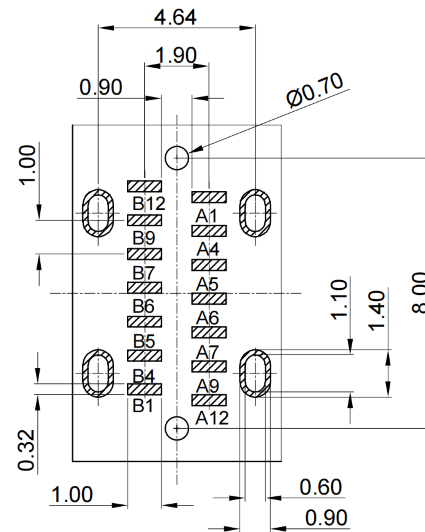
RECOMMENDED PCB LAYOUT TOLERANCE: ±0.05
