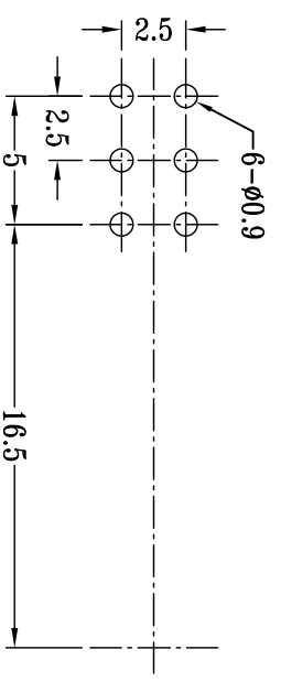
P.C.B LAYOUT BOTTOM VIEW
