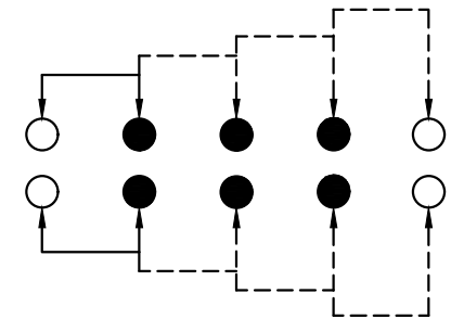
SCHEMATIC (NON-SHORTING)
