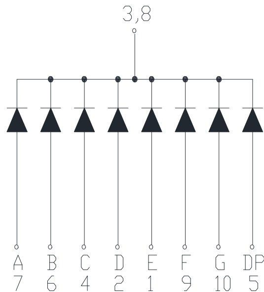
Common Cathode
