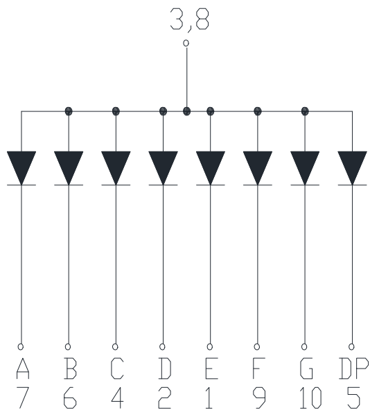
Common Anode
