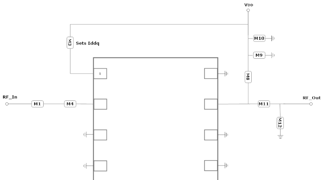
GRF2074 Application Schematic (SDARS)
