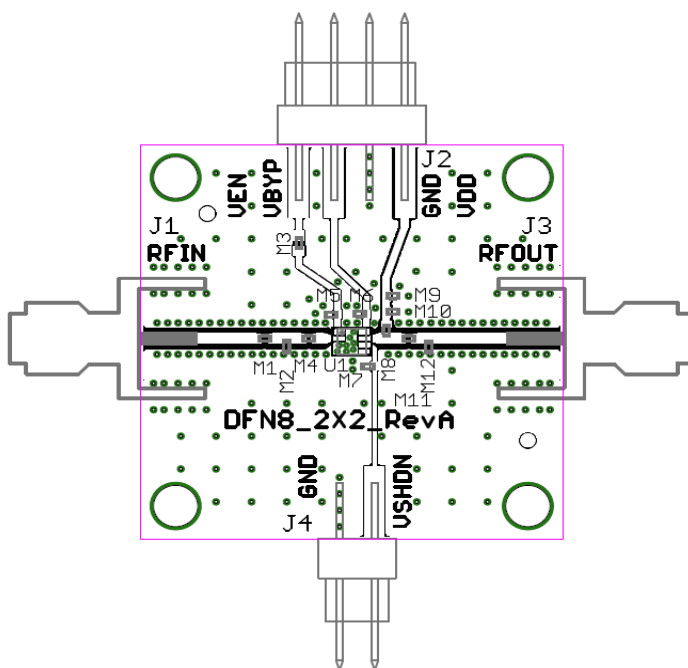
GRF2074 EVB Assembly Drawing
