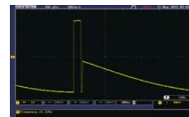
ISO7637-2 TP2B
