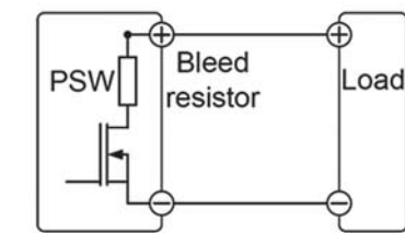
PSW-Series Built-in Bleed Resistor
