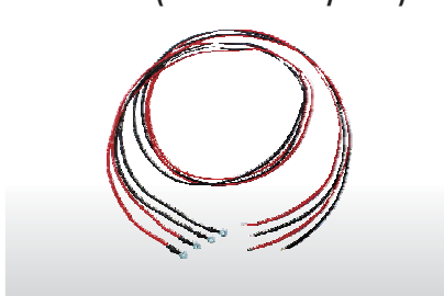
GTL-130 Test lead, 1200mm, 18AWG, UL 3239 (for PSW 250V/800V)
