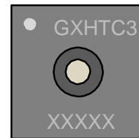
Figure 8 Laser marking on GXHTC3, the top line with the pin-1 indicator and the sensor type, the bottom line with the 5-digit alphanumeric tracking code.
