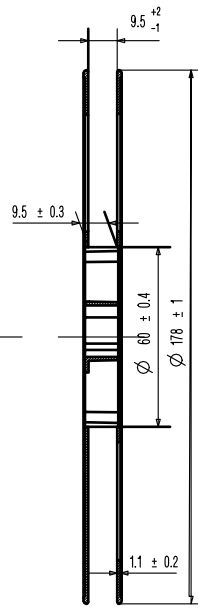
SECTION AE - AE
