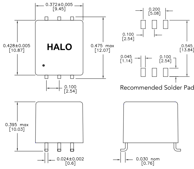
Dimensions: Inch[mm]
