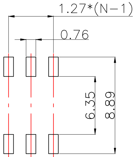
[P.C.B.LAYOUT]
